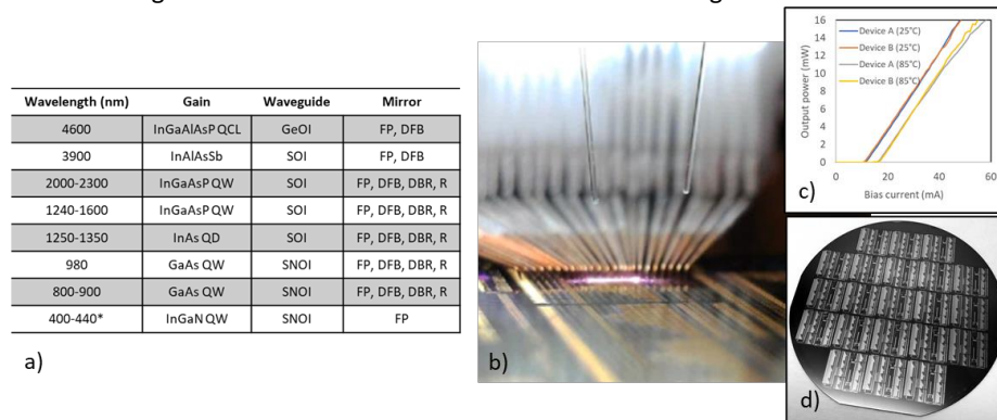
Figure 2. (a) Summary of laser technologies on silicon (GeOI – germanium on insulator, SOI – silicon on insulator, SNOI – silicon-nitride on insulator, R stands for one or more rings), (b) Automated wafer scale testing of lasers captured with operation Si camera showing light emission below Si bandgap, (c) Exemplary LIV curves showing very good laser performance (the wavelength of is 980 nm) and (d) Heterogeneous GaAs-on-SiN wafer with multiple active components including lasers, amplifiers, photodetectors and tuners.
