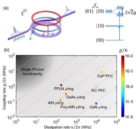
Figure 3. (a) A \chi(2) cavity with single-photon nonlinearity based on a periodically poled lithium niobate microring and its schematic energy level diagram (right panel). The anharmonicity of the nonlinear system is determined by the energy level splitting relative to their widths. (b) The coupling rate g , dissipation rate \kappa as well as the corresponding single-photon nonlinearity FOM demonstrated in various integrated \chi(2) cavities. \mu ring, microring; PhC, photonic crystal.
