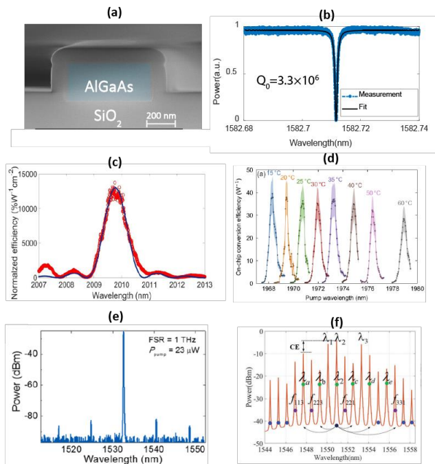
Figure 1. Demonstrations on (Al)GaAsOI platform. (a) SEM image of the cross section of an AlGaAsOI waveguide. (b) Transmission spectrum of an AlGaAs resonator. The extracted Q is 3.3 \times 10^6 . (c) The transfer function of SHG normalized efficiency for a GaAsOI waveguide. (d) SHG spectra under different temperatures by a GaAsOI waveguide, whose normalized efficiency is > 40,000\% W^{-1}cm^{-2} . (e) The generated frequency comb lines from an AlGaAs resonator under 23 \mu W power. (f) Frequency conversion for communication experiment by an AlGaAsOI waveguide.
