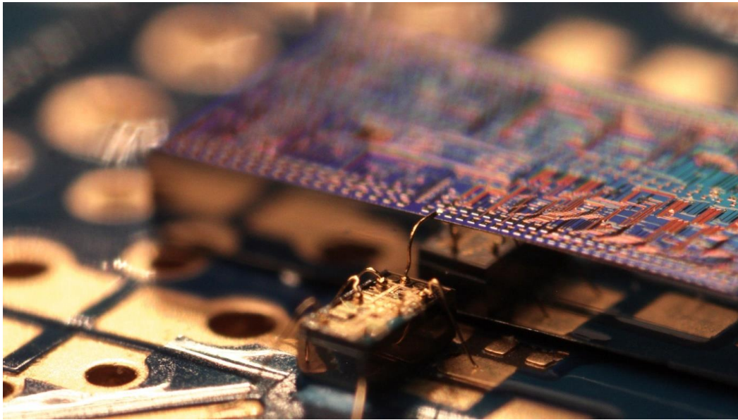
Figure 1. An integrated electronics die directly wire-bonded with a silicon photonics integrated circuit reduces total device capacitance, thereby enabling in this instance [11] a high bandwidth homodyne detection for squeezed light detection on-chip. [Photo credit: Joel Tasker, University of Bristol].
