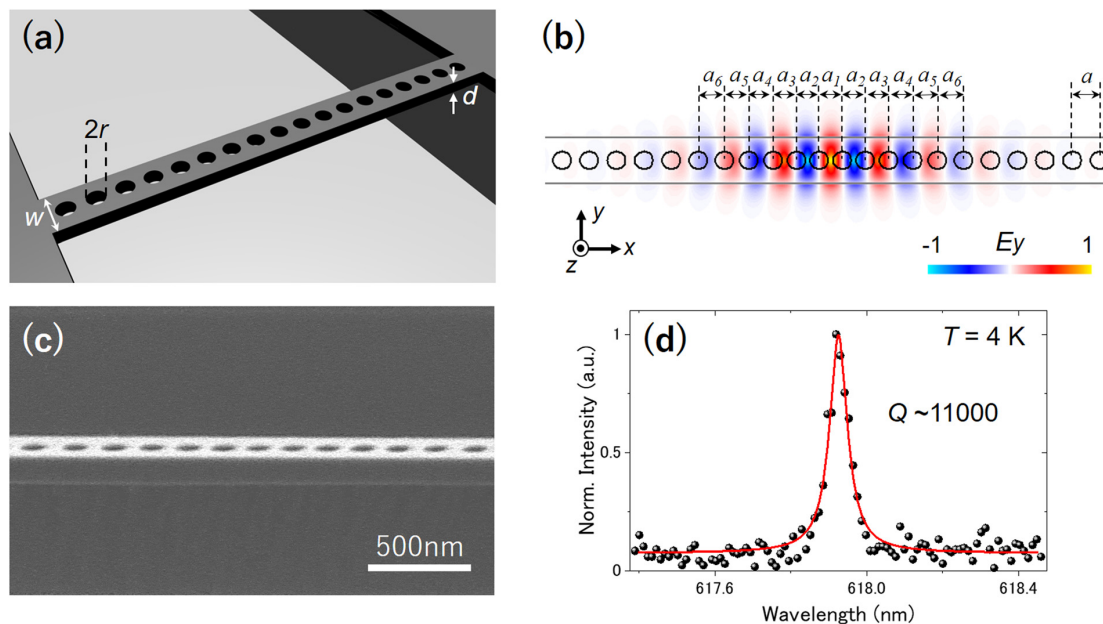
FIG. 1. (a) Schematic view of the free-standing 1D PhC nanobeam cavity on bulk single-crystal diamond. (b) Calculated electric field distribution for the fundamental cavity mode with a theoretical Q factor of \sim 6 \times 10^5 . The quadratic modulation of the air hole positions ( a_1 \sim a_6 ) is applied near the center of the waveguide to form the cavity. (c) Scanning electron microscope image of a fabricated cavity. (d) Selected PL spectrum of a cavity with a = 188 nm, exhibiting the highest Q factor among the 153 measured cavities. The red solid line is a fitting curve.
