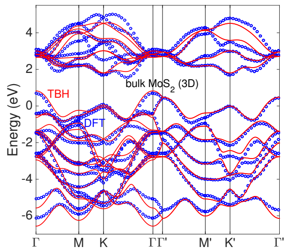
FIG. 7. Band structure of the bulk, 3D crystal of MoS 2 , in the 2H structure, as obtained from DFT calculations (blue circles) and from the TBH (red lines) derived from the bilayer system (including inter-layer coupling). The symbols \Gamma -M-K- \Gamma correspond to k_z = 0 , while those with prime correspond to k_z = \pi/c .
