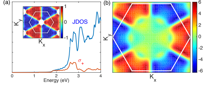
FIG. 9. MoS 2 TBH: (a) \sigma_+ absorption and comparison with joint density of states (JDOS); the inset shows the k -resolved degree of polarization \eta(\mathbf{k}) . (b) Berry curvature in units of \text{\AA}^2 .
