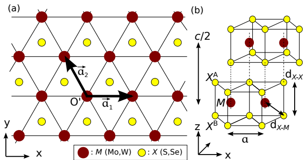
FIG. 1. (a) Top view of a single layer TMDC crystal structure with hexagonal primitive vectors \mathbf{a}_1 and \mathbf{a}_2 . The smaller yellow circles represent the two chalcogen atoms separated by d_{X-X} in the z direction and the larger brown circles the metal atoms. (b) Perspective side view for the TMDC 2H crystal structure composed of X^A -M- X^B monolayers with a the in-plane lattice constant and c/2 the separation between two units along the \hat{z} -axis.
