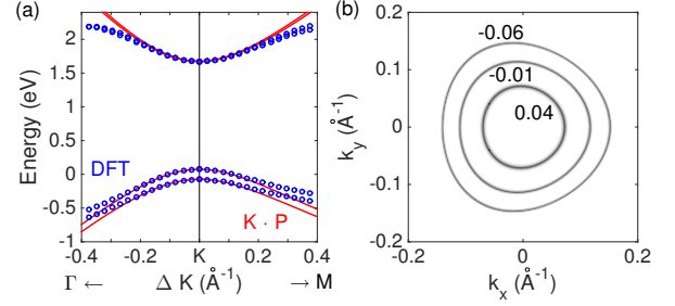
FIG. 8. (a) Comparison of the \mathbf{k} \cdot \mathbf{p} hamiltonian (red lines) and the DFT results (blue dots) for the MoS 2 monolayer with spin-orbit coupling at \mathbf{K}_{+} . (b) Energy contours in eV for the highest valence band centered at \mathbf{K}_{+} . The deviation from spherical symmetry is due to the f_4 term.
