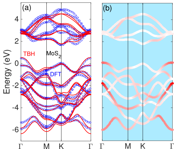
FIG. 6. (a) TBH band structure (red lines) along \Gamma -M-K- \Gamma and the comparison with DFT results (blue circles) for a MoS 2 bilayer in the 2H structure. (b) The overlap matrix element strength between two layers with the interlayer coupling hamiltonian that leads to splitting of single-layer states, on a scale from red (strongest) to white (weakest).
