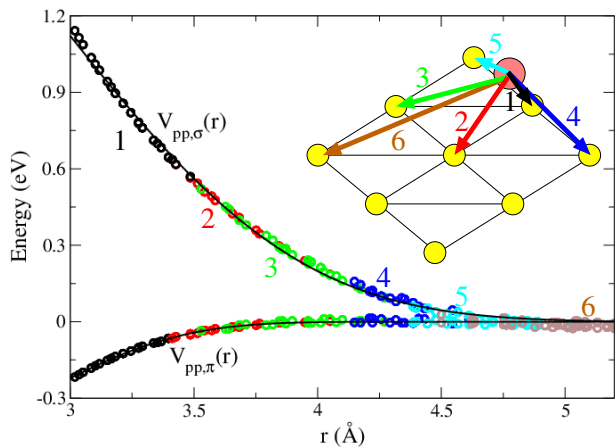
FIG. 5. V_{pp,\sigma}(r) (upper) and V_{pp,\pi}(r) (lower) for interlayer pairs as function of the pair distance r in a MoS 2 bilayer unit. Black, red, green, blue, cyan, brown are data points from 1st, 2nd, 3rd, 4th, 5th, 6th nearest distances. The solid black lines going through the points are the fits as obtained from Eq. 17. The inset is the perspective view for the interlayer coupling between one of the S atom on the top unit (orange) to all other S atoms on the bottom unit (yellow).
