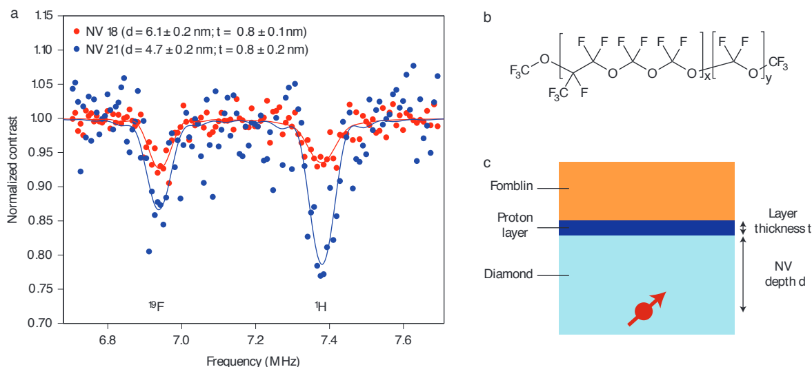
Figure 5 | Determination of surface proton layer thickness. a, NMR signal from Fomblin Y oil on the diamond surface measured with two NV centres separated by \sim 5 \mu\text{m} . NV depths are presented, as calculated from the lineshape model (see Supplementary Methods). b, Chemical structure of Fomblin Y oil. c, Description of the hypothesized sample structure resulting from Fomblin Y oil floating above a thin layer of adsorbed hydrocarbons or water on the diamond surface.
