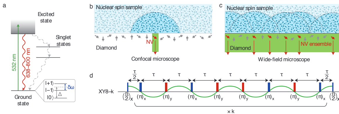
Figure 1 | NV NMR experiment. a, NV centre energy level diagram (see Supplementary Methods for details). b, A confocal microscope interrogates a single shallow NV centre, which detects NMR signals from a few-nanometre region of sample on the diamond surface. c, A wide-field microscope images fluorescence from a shallow, high-density layer of NV centres allowing detection of NMR signals from overlapping nanoscale regions of sample on the diamond surface. Only NV centres of the same orientation (shown in red), aligned along an externally applied static magnetic field, B_0 , contribute to the ensemble NV NMR signal. d, Larmor precessing nuclear spins in the sample produce an effective a.c. magnetic field (such as the one shown by the green line) that is detected by NV sensors in a frequency-selective manner using an XY8- k pulse sequence.
